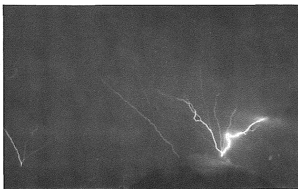
Figure 2 - Upward strokes from both towers (right) and from Monte Sighignola (left)
