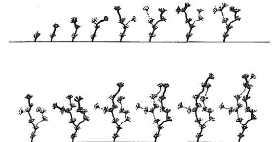
Figure 4 - Upward stroke from the negative top of the tower towards a positive cloud
