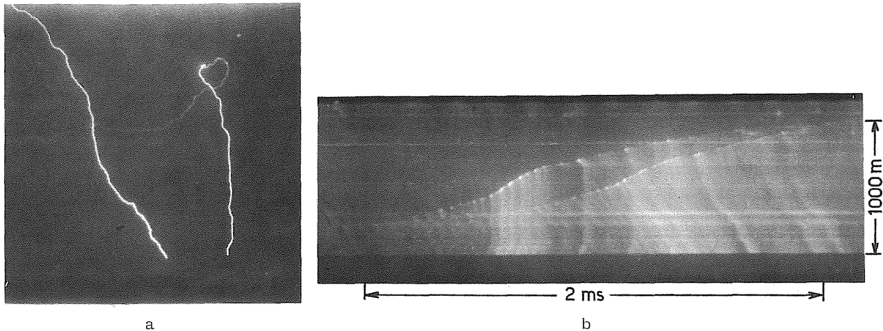
Figure 5 - Upward strokes from both towers, from positive top of the tower to negative cloud
