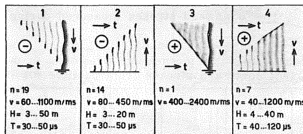
Figure 6 - The growth of negative and positive streamers
