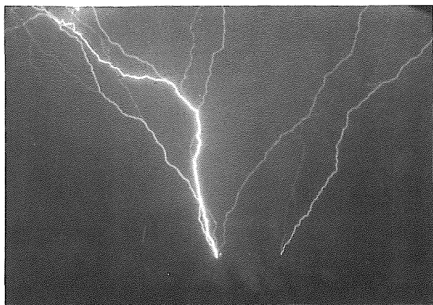
Figure 1 - Upward strokes, simultaneous from both towers
