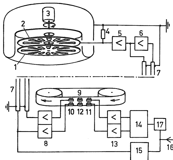
Figure 9 - Schematic representation of the whole set of equipment used for recording the field
