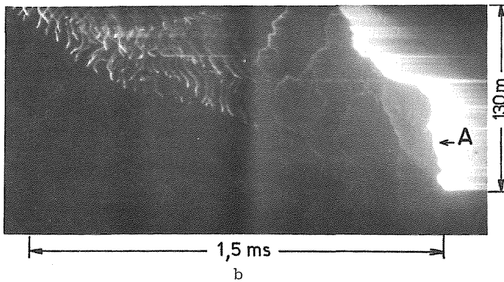
Figure 3 - Downward stroke from a negative cloud, striking the tower 400 m away
